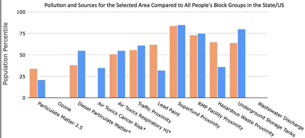
Pollution and Sources (*A mid-point of the percentile range is used to chart each of the air toxics parameters.)
